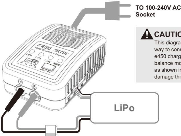
CONNECTION DIAGRAM
